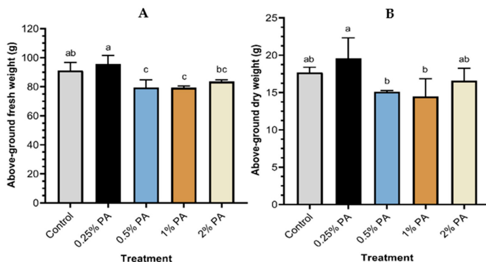
Figure 1. Pyroligneous acid effect on tomato plant above-ground biomass: (A) fresh weight and (B) dry weight. Values are the means of four replicates and different lowercase alphabetical letters indicate significant ( p < 0.05 ) difference according to Fisher's least significant difference (LSD) post hoc test. Error bars show the standard deviations.
